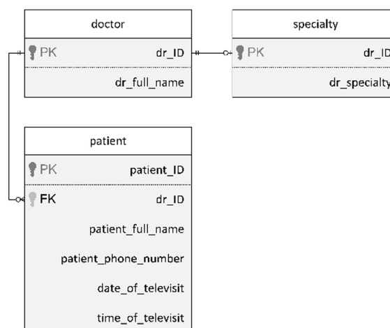
Figure 1: The Entity relationship diagram shows the structure of and the relationship between the doctor, the specialty, and the patient datasets.
