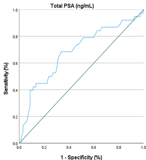
Figure 1: The receiver operating characteristic (ROC) curve illustrates the diagnostic accuracy of total prostate-specific antigen (PSA) in predicting lymph node invasion (LNI) in patients with intermediate-risk prostate cancer (PCa).
