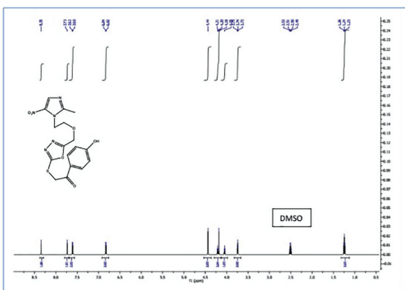
Figure S9: 1 H NMR spectra of compound 10d
