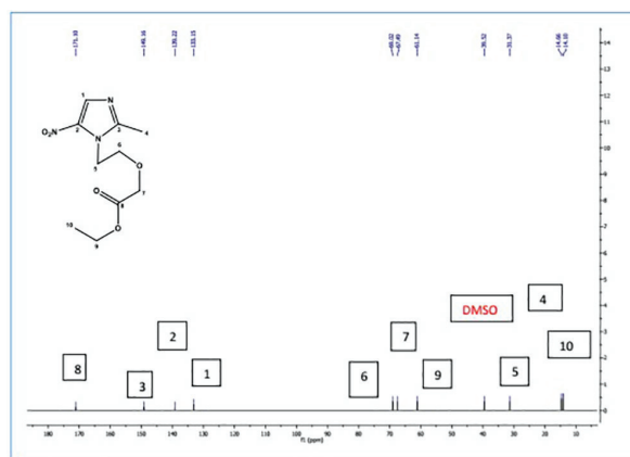
Figure S2: 13 C NMR spectra of compound 7
