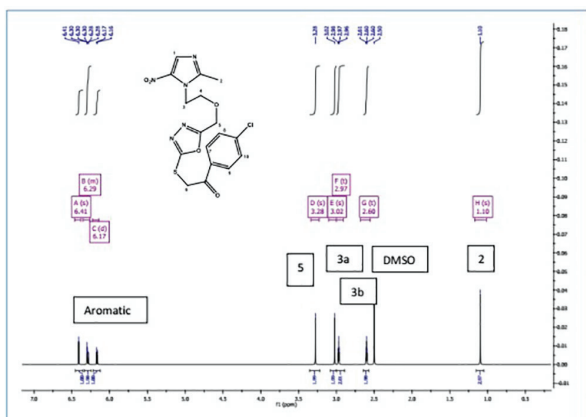
Figure S5: 1 H NMR spectra of compound 10a
