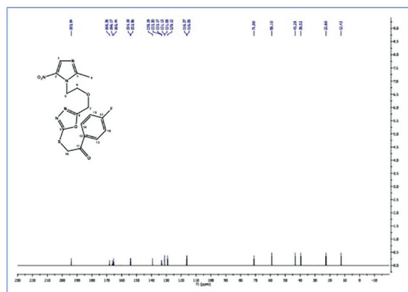
Figure S8: 13 C NMR spectra of compound 10c
