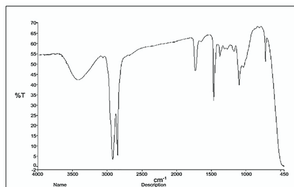
Figure S18: I.R Spectrum of compound 10f
