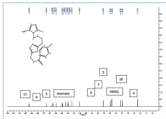
Figure S6: 13 C NMR spectra of compound 10a
