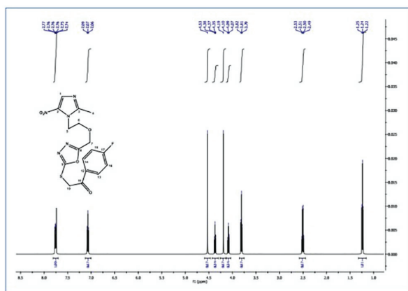
Figure S7: 1 H NMR spectra of compound 10c
