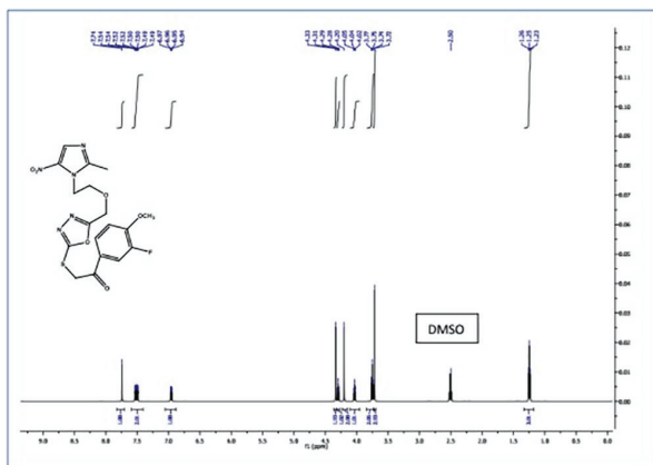
Figure S13: 1 H NMR spectra of compound 10f
