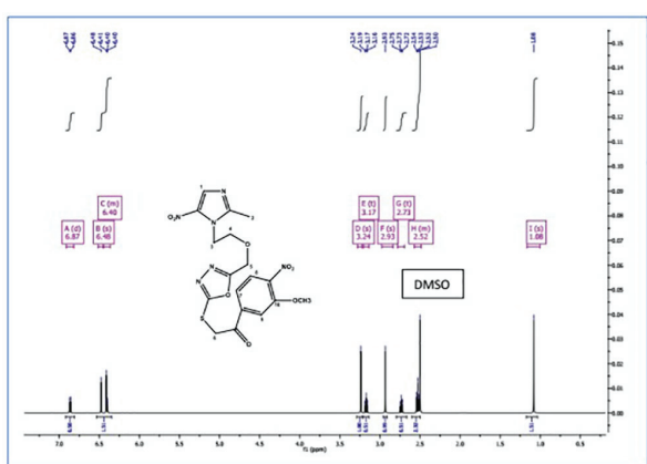
Figure S11: 1 H NMR spectra of compound 10e
