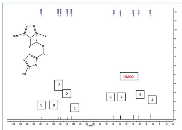
Figure S4: 13 C NMR spectra of compound 9
