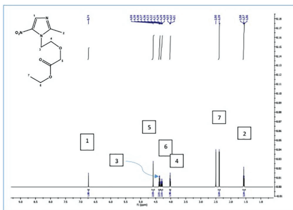
Figure S1: 1 H NMR spectra of compound 7
