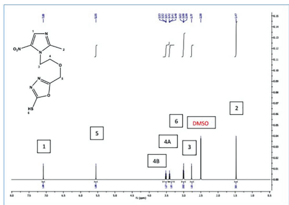
Figure S3: 1 H NMR spectra of compound 9
