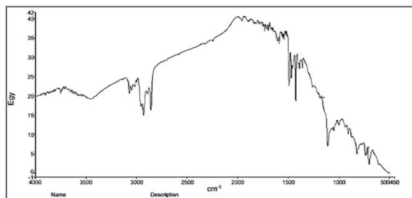
Figure S17: I.R Spectrum of compound 10e
