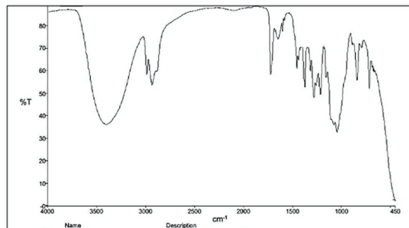
Figure S16: I.R Spectrum of compound 10d
