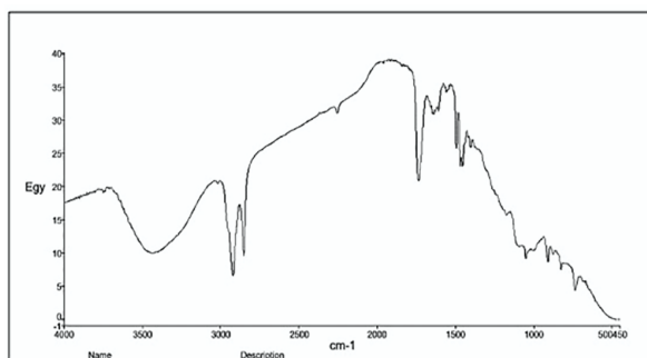
Figure S15: I.R Spectrum of compound 10a
