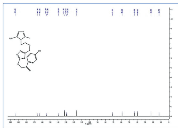
Figure S10: 13 C NMR spectra of compound 10d
