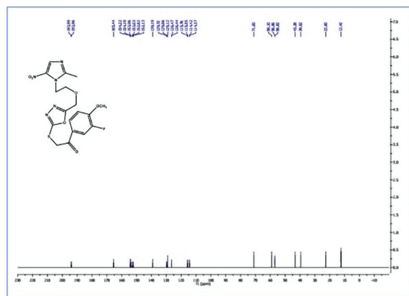
Figure S14: 13 C NMR spectra of compound 10f
