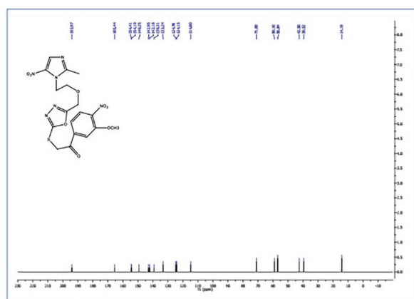
Figure S12: 13 C NMR spectra of compound 10e
